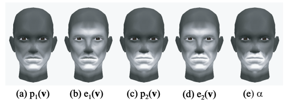
Figure 14: Importance distributions
